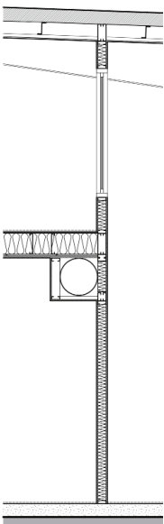
04 / Wall Section B Bike Studio and Office
