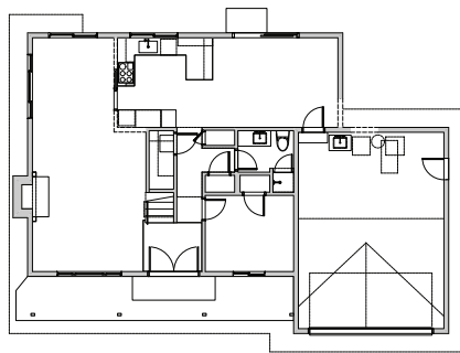
Existing 1st Floor
